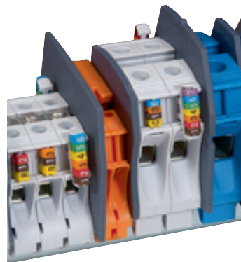
Terminal block with CAB 3 markers and label holders
