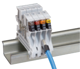
Example of single/double ferrules on cables
